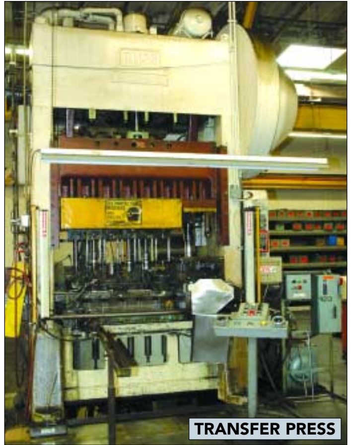
100-TON BLISS STRAIGHT SIDE PRESS, MDL. S2-100
