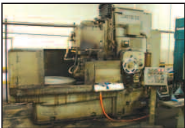
MATTISON "BLANCHARD" TYPE GRINDER
