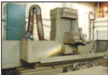
MATTISON 18" X 75" SURFACE GRINDER
