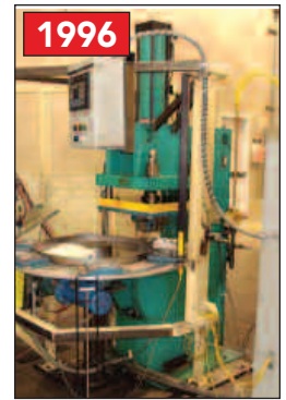
VIEWS OF TOX PRESSOTECHNIK 30-TON PNEUMATIC PRESSES
