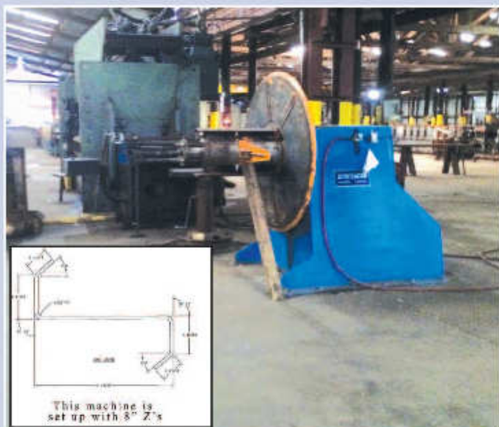
Purlin Roll Former Line, Jamco Decoiler, Strainer, HTC Shear, Omega Roll Former, # Stands 12
