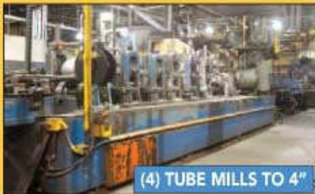
AEF 2-1/2" TUBE MILL
