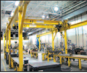
FREE STANDING BRIDGE CRANE
