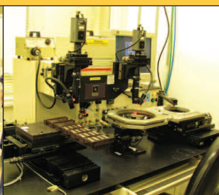
Dataconn 2200APM+ Single Gantry Auto. Die Bonder. S/N 95022141103, Mfg. Date 2003
