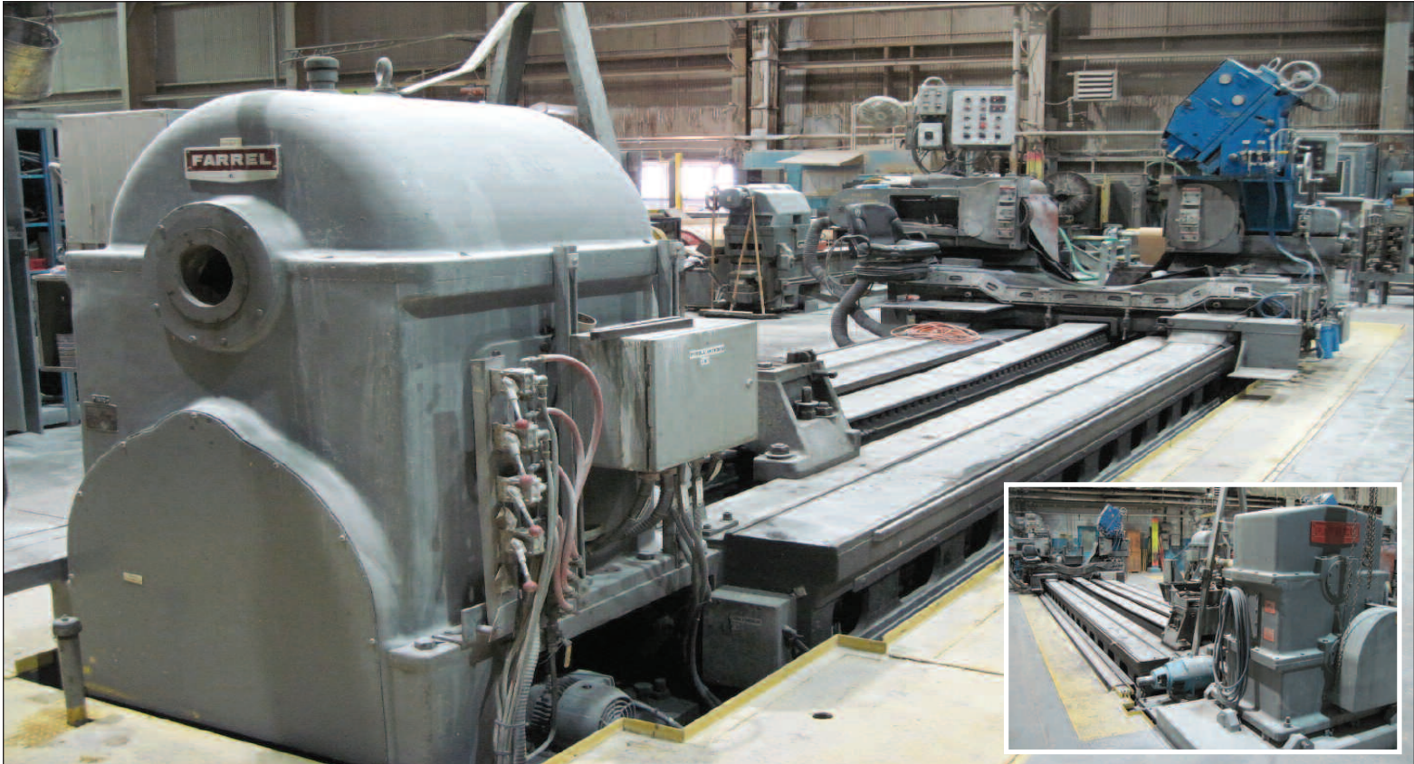
(2) Farrel Two Wheel Roll Grinders
