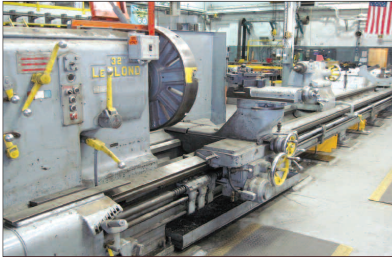
LeBlond Engine Lathe, S/N NK928
