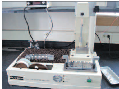
Huygen Internal Bond Tester
