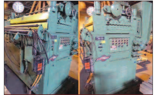
48" x 0.035" Littell Leveler/Straightener
