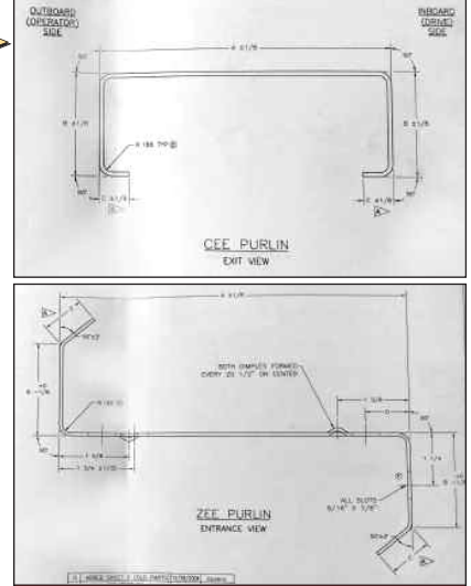
CEE & ZEE Profile
