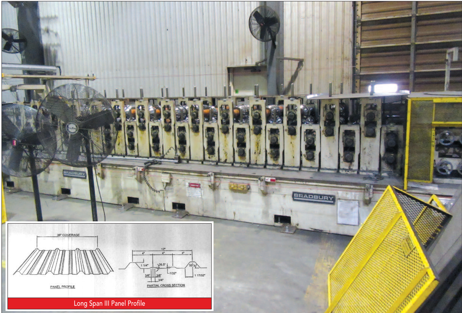
Bradbury Double High Metal Siding Panel Rollformer
