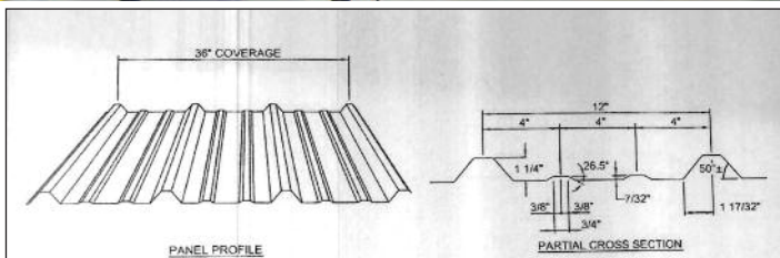
Long Span III Panel Profile
