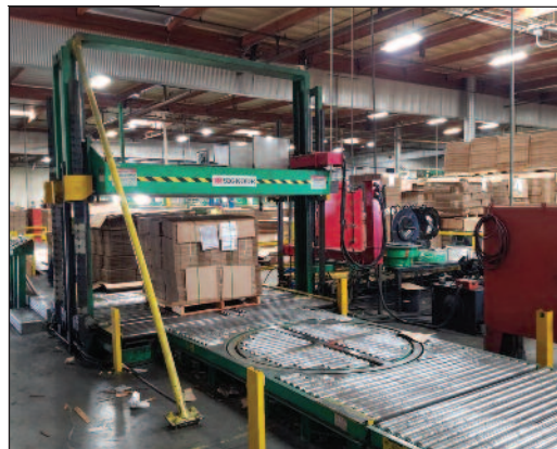
Signode Three-Head Unitizer
