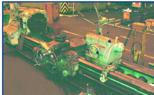
AMERICAN PACEMAKER Engine Lathe, 40"x123"
