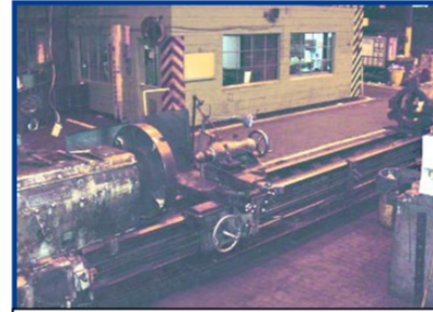
MONARCH Engine Lathe, 36.5"x192"
