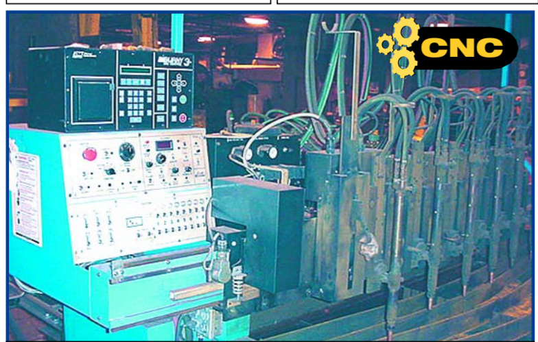
C&G System Burning Machine, 6-Head w/Plasma
