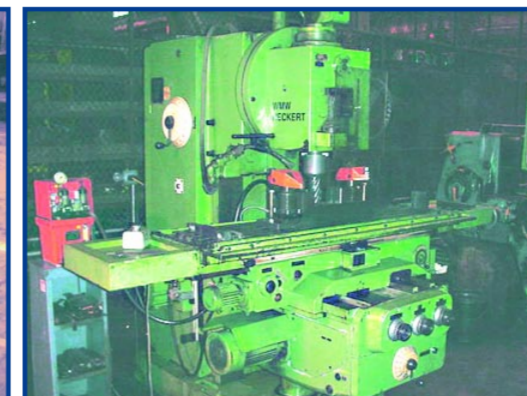
HECKERT Universal Vertical Mill, Mdl. F400E
